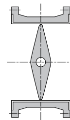
Centric operating principle.
