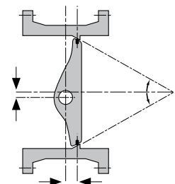
Butterfly valves 567: Double eccentric operating principle.
