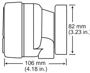
SIDE VIEW Field Mount w/ 8050 Universal base
